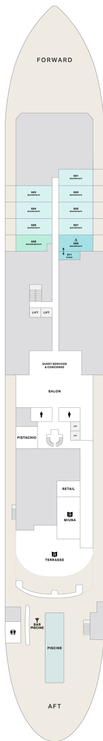
DECK 5
